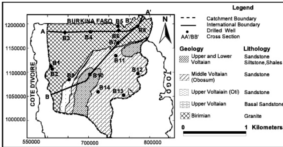
Fig.2 : Map Showing Geology and Cross Sections Of the White Volta Basin
