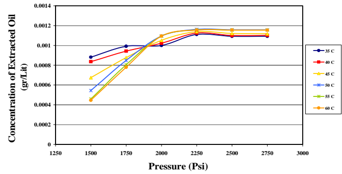
Fig 4. Concentration of Extracted Oil as a function of Pressure
