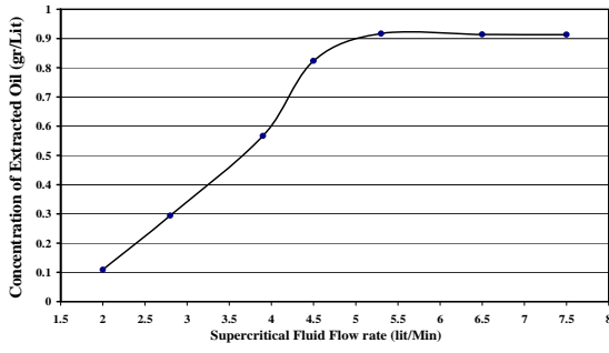
Fig 1. Concentration of Extracted Oil as a function of S.C.F Flow Rate
