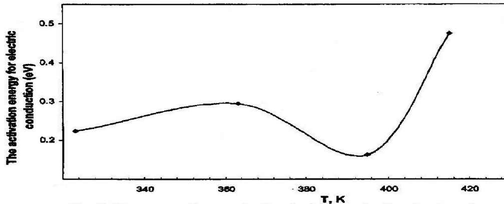
Fig. 8. The energy diagram for the electric conduction mechanism during the transformation in the amorphous DPC samples with temperature.
