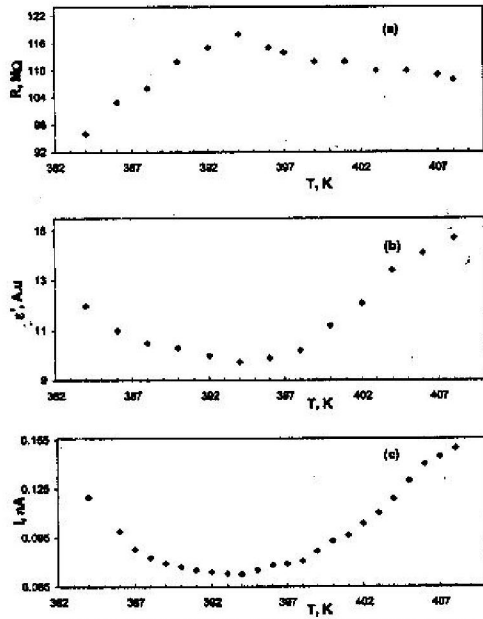
Fig. (6a - c) : The Variation of the electrical resistance (a), the dielectric constant (b) and the pyroelectric current (c) with temperature for amorphous DPC samples during the heating transformations.
