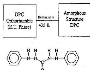
Fig. 1. The structure of the diphenyl carbazide compound.
