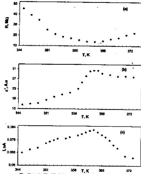
Fig. (5a - c) : The Variation of the electrical resistance (a), the dielectric constant (b) and the pyroelectric current (c) with temperature for amorphous DPC samples during the heating transformations.
