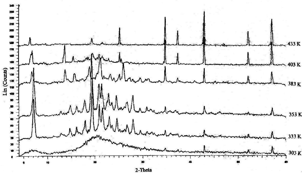
Fig. 9 X-ray diffraction patterns for the polymorphism of amorphous DPC at different temperatures (303, 333, 353, 383, 403, 433 K).
