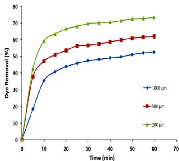
Figure 3: Effect of variation in size of alginate beads on dye removal
