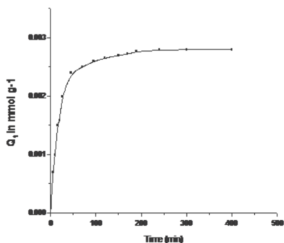
Figure 4: Adsorbed amount of methylene blue by alginate beads as a function of time
