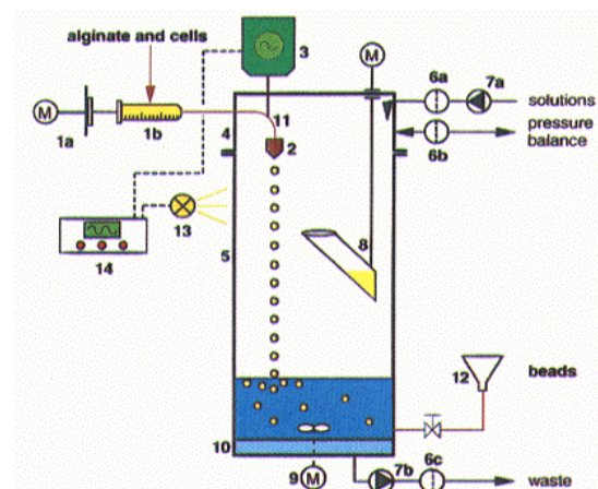
Figure 1: Schematic diagram represents the formation of alginate beads using encapsulator.
