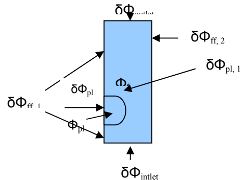
Figure 6: Schematic diagram of the domain that will be modeled.
