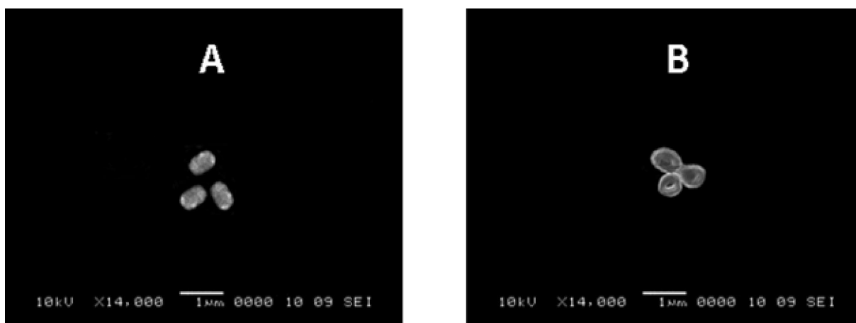
Figure 2. Scanning electron microscopic micrograph of B. subtilis ATCC 6633 spores; untreated (A) or treated (B) with ozone conc. ( 5.0 \text{ g/m}^3 ) at 37^\circ\text{C} for 1 min. Note that the surface layer and the outer spore coat are the structures most apparently damaged by ozone treatment
