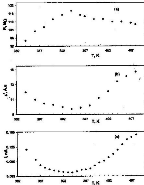
Fig. (6a - c): The Variation of the electrical resistance (a), the dielectric constant (b) and the pyroelectric current (c) with temperature for amorphous DPC samples during the heating transformations.
