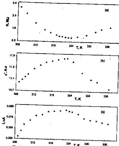
Fig. (4a - c): The Variation of the electrical resistance (a), the dielectric constant (b) and the pyroelectric current (c) with temperature for amorphous DPC samples during the heating transformations.
