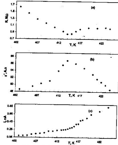
Fig. (7a - c): The Variation of the electrical resistance (a), the dielectric constant (b) and the pyroelectric current (c) with temperature for amorphous DPC samples during the heating transformations.
