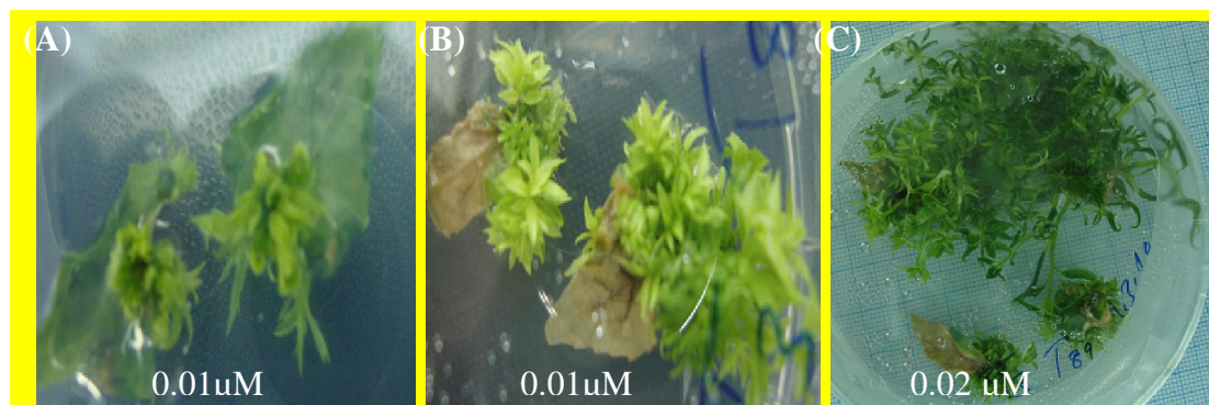
Fig (1): Direct shoot regeneration obtained from leaves on MS medium supplemented with TDZ. (A and B) development of shoot initials on leaves of P. tremula x P. tremuloides after 4 and 8 weeks in culture, respectively. (C) Adventitious shoots formed on leaves of P. tremula x P. tremuloides eight weeks after the initial culture.
