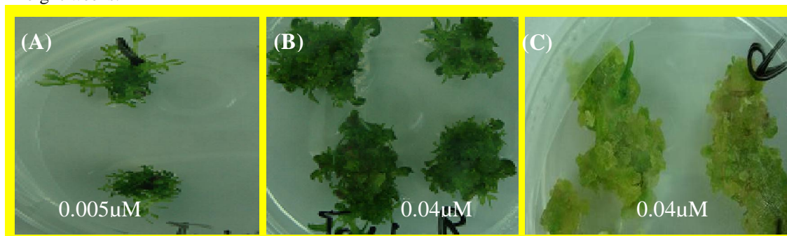
Fig (3): Adventitious shoot regeneration from root explants on MS medium supplemented with TDZ. (A and B) Adventitious shoots of P. tremula after 4 and 8 weeks in culture, respectively and (C) Callus formation and development of shoot initials of P. alba after eight weeks.
