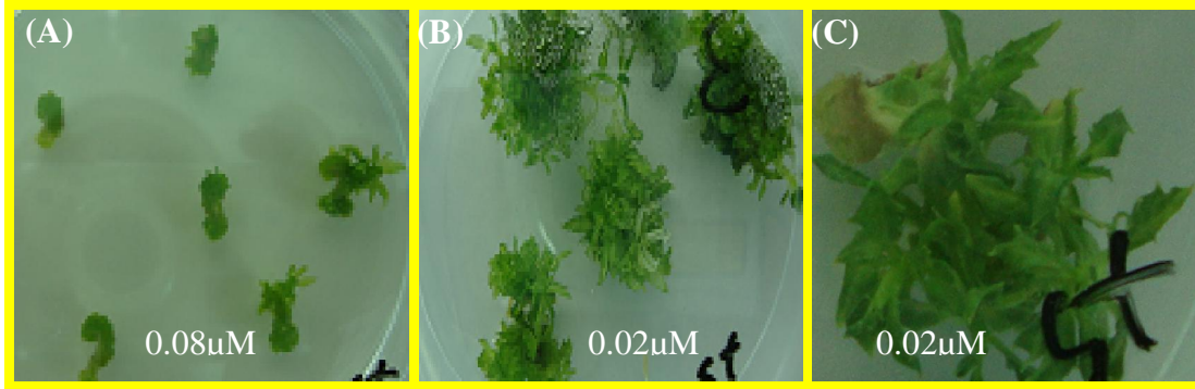
Fig (2): Direct shoot regeneration obtained from stem internode explants on MS medium supplemented with TDZ. (A and B) Adventitious shoots of P. tremula x P. tremuloides after 4 and 8 weeks in culture, respectively and (C) Adventitious shoots of P. alba after eight weeks.
