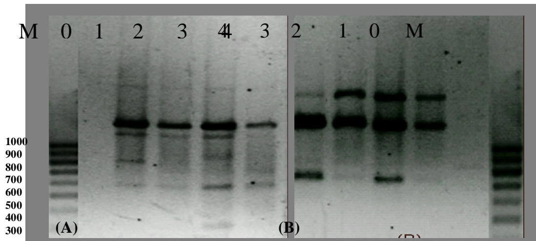
Fig (4): (A and B) Electrophoresis pattern of DNA amplification products obtained after direct shoot regeneration from stem internode and root explants of P. tremula x P. tremuloides and P. tremula , with primers A6 and A7, respectively, Lanes 2, 3 and 4 refer to sample plants, 1 is the control plant, 0 refers to the negative control of PCR and M refers to the DNA marker.
