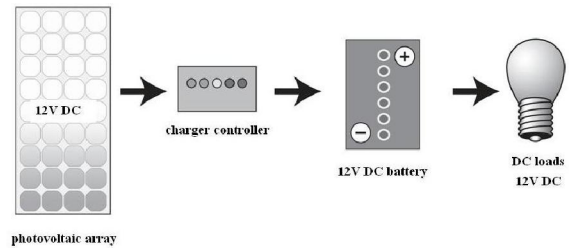
Fig 3- DC system with storage battery
