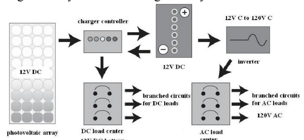
Fig 4- A system with DC and AC loads
