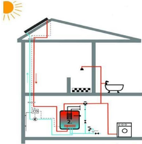
Fig 6- The system providing hot water for consumption in the solar package
