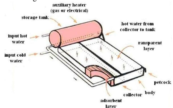
Fig 7- Closed-cycle thermo siphon system
