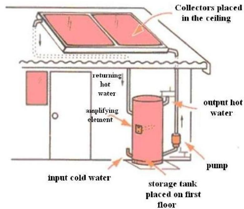
Fig 9- Compulsory circulating system
