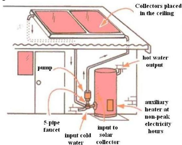
Fig 12- retrofits (electricity at non-peak hours)
