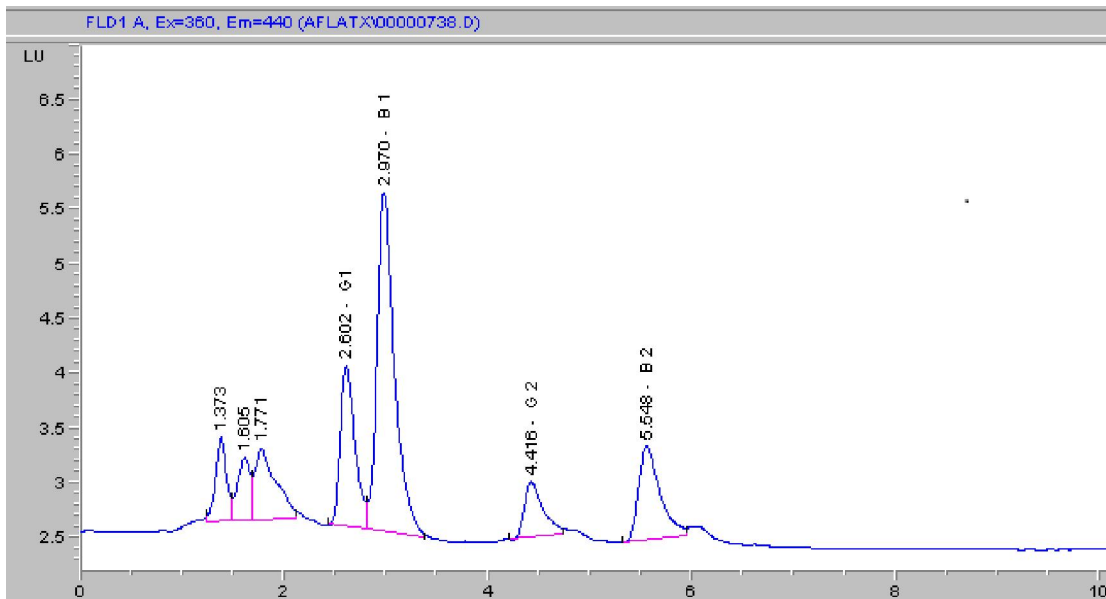
Figure (2): High Performance Liquid Chromatogram of a standard of aflatoxins (AFG 1 , AFB 1 , AFG 2 and AFB 2 )
