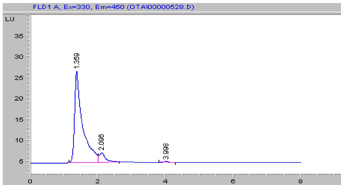
Figure (3): High Performance Liquid Chromatogram of a negative sample of aflatoxins (AFG 1 , AFB 1 , AFG 2 and AFB 2 )
