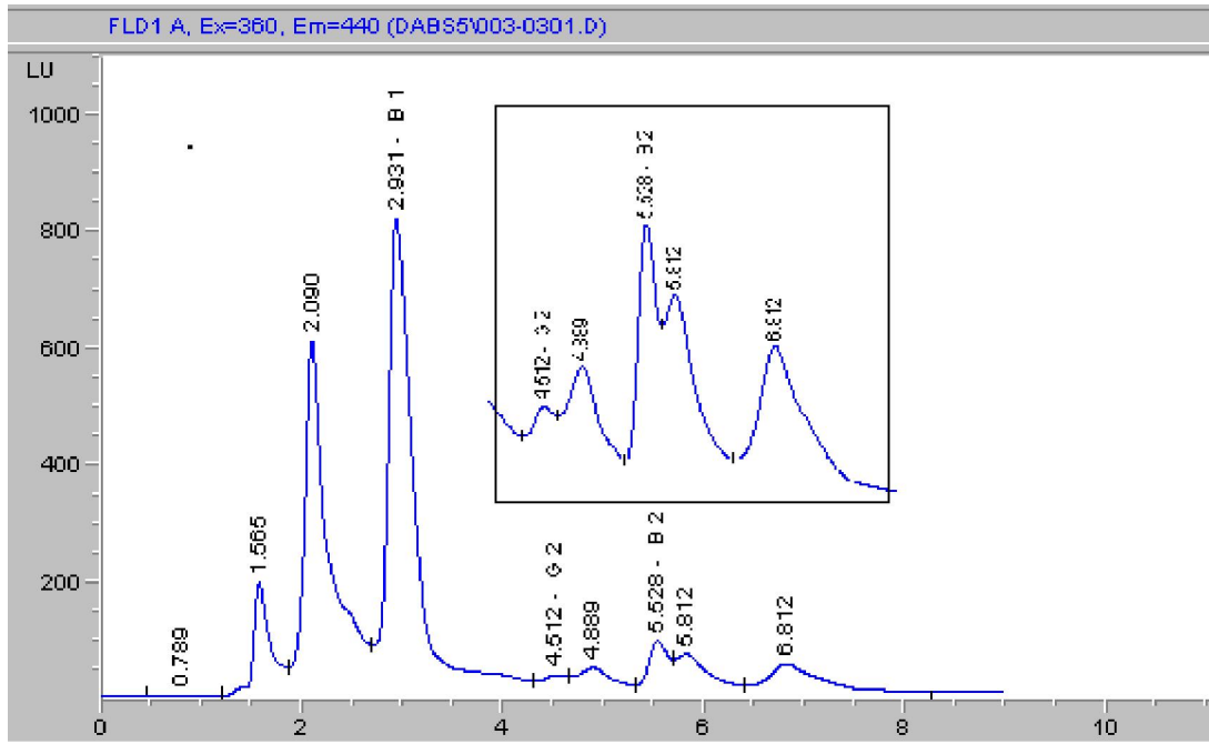
Figure (1): High Performance Liquid Chromatogram of a positive sample of aflatoxins (AFG 1 , AFB 1 , AFG 2 and AFB 2 )
