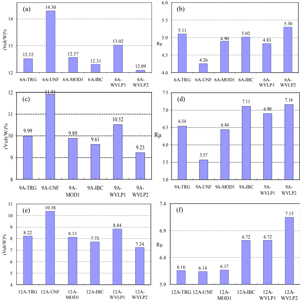
Figure 4. Pushover Analysis Results: (a) 6-Story V_{ult}/W Ratio, (b) 6-Story R_{\mu} Factor, (c) 9-Story V_{ult}/W Ratio, (d) 9-Story R_{\mu} Factor, (e) 12-Story V_{ult}/W Ratio, and (f) 12-Story R_{\mu} Factor
