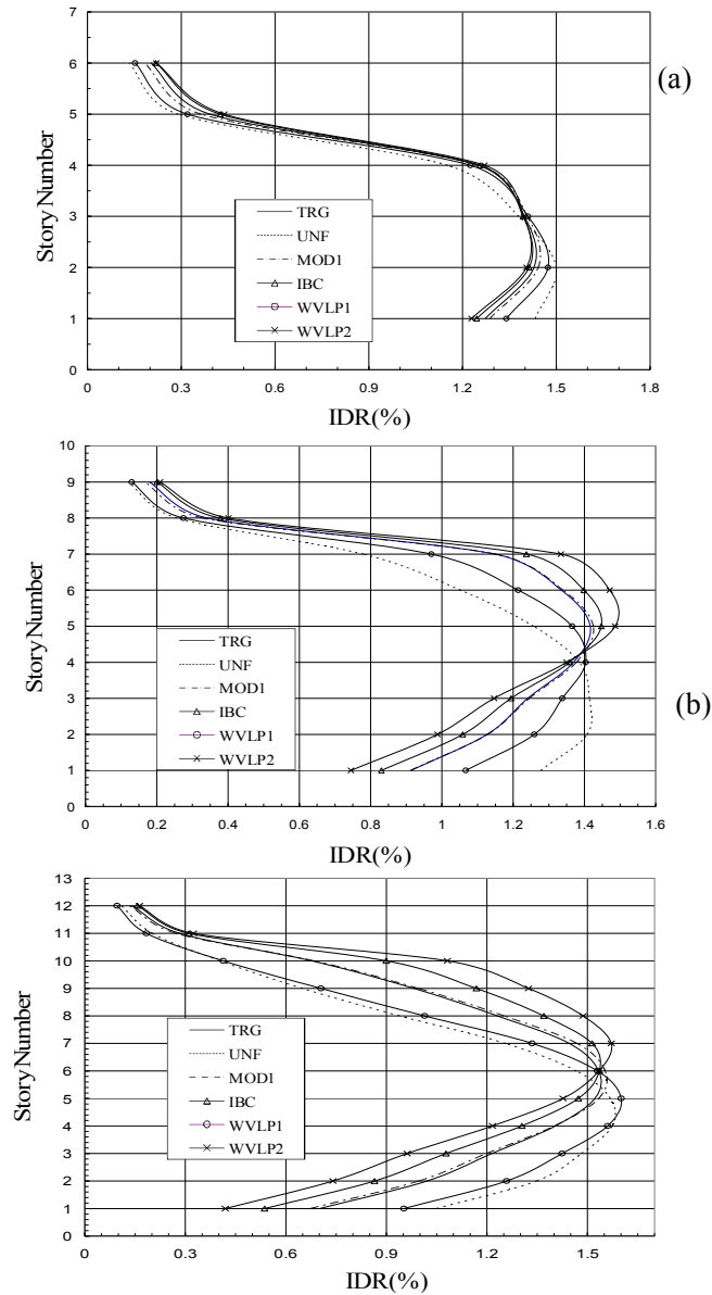
Figure 5. Pushover Analysis Results: (a) 6-Story IDR, (b) 9-Story IDR, and (c) 12-Story IDR
