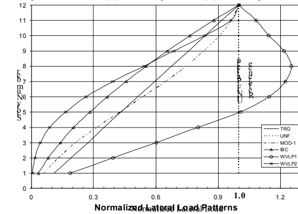
Figure 6. Normalized Lateral Load Patterns for 12-Story Model
