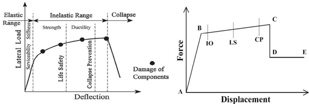
Figure 1. (a) Typical Performance Curve for the Structure, and (b) Typical Plastic Hinge Behaviour (FEMA 356)
