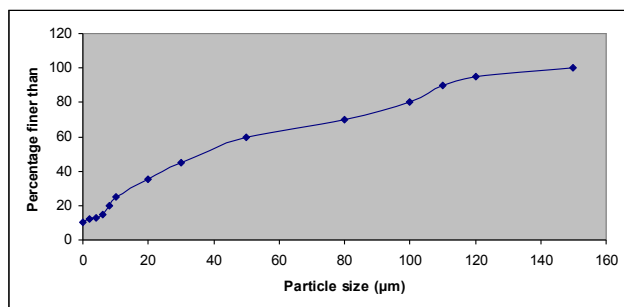
Fig. 1. Illustration of cement particles' distribution.
