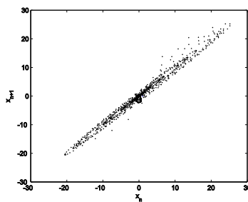
Figure 8: The points (x_k, x_{k+1}) for 2000 iterations when \varepsilon = -13
