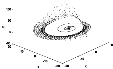
Figure 8: \|X\| in 2-dimensional and 3-dimensional space all 2000 iterations when \varepsilon = -13
