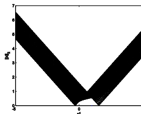
Figure 3: \|X\| for the last 100 iterations when a = 4, b = 1
