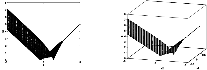
Figure 5: \|X\| for the last 100 iterations when \alpha = 4, b = 1 and \varepsilon = (\varepsilon_1, 0.1\varepsilon_1)
