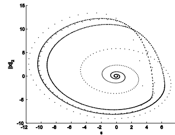
Figure 8: \|X\| in 2-dimensional and 3-dimensional space all 2000 iterations when \varepsilon = -13
