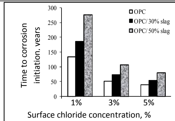
Fig. 5. Time to corrosion initiation of OPC/slag concrete (concrete cover equal to 0.07 m,
