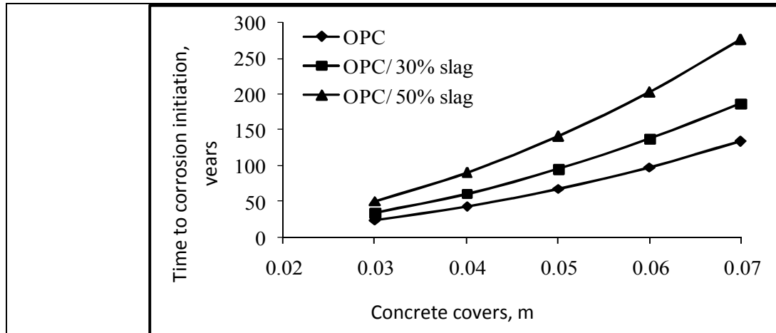
Fig. 6. Time to corrosion initiation of OPC/slag concrete (surface chloride concentration of 1%)
