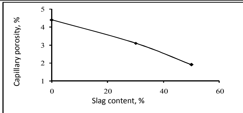
Fig. 3. Capillary porosity of OPC/slag pastes.
