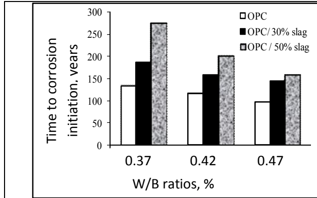
Fig. 4. Time to corrosion initiation of OPC/slag concrete (concrete cover equal to 0.07 m, surface chloride concentration of 1%)
