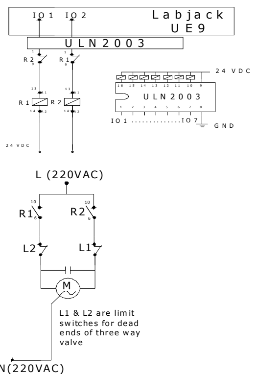
Figure 7. Interfacing the AC motor with LabJack UE9 by means of ULN2003A chip to change the motor rotating direction, the figure shows the setting of limit switches for both dead ends of the valve.
