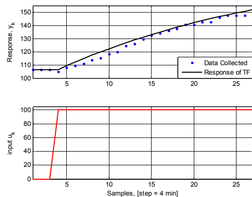
Figure 13. The response of the model (8), with respect to data collected at step input (100%), using equation error method. The model parameters are
