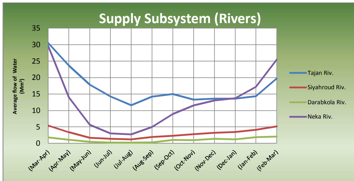
Figure 2. Diagram of flows of 4 rivers in a year
