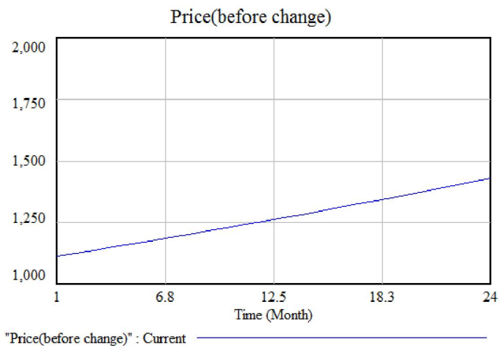
Figure 11. Third strategy for water price, price increases by inflation
