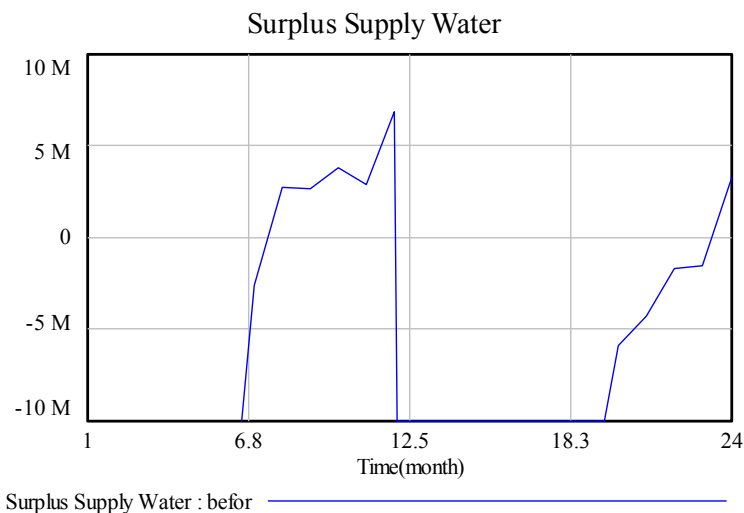
Figure 14. Surplus supply water and its changing in modeling horizon
