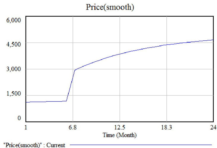
Figure 9. First strategy for water price, price increases smoothly
