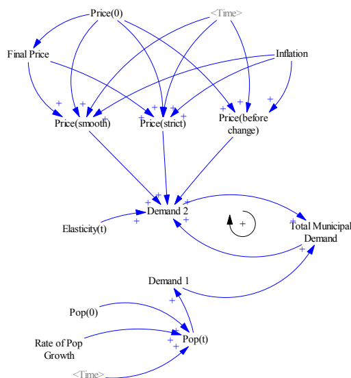
Figure 5. Causal diagram of municipal Demand
