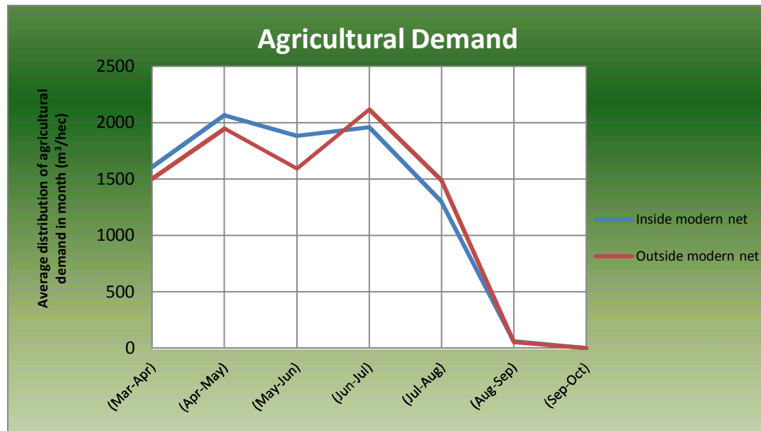
Figure 3. Diagram of Agricultural Demand
