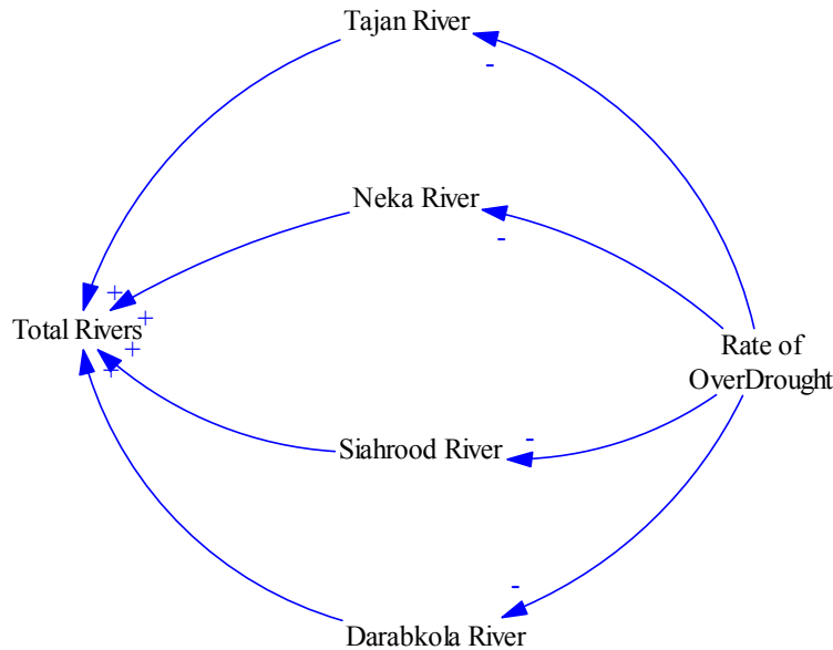
Figure 6. Causal diagram of supply subsystem
