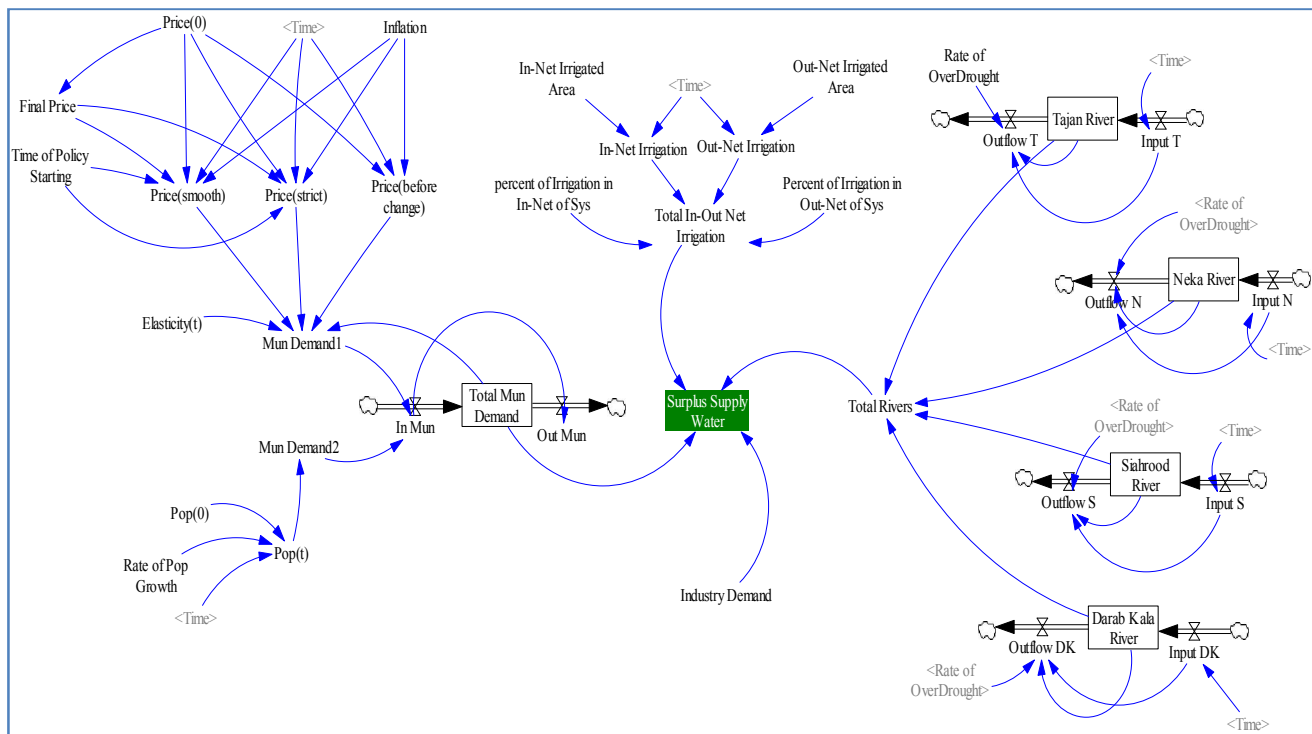
Figure 7. Flow diagram of model
